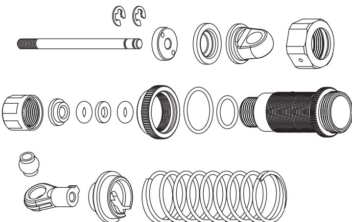
Front Shock Absorber 2PCS
