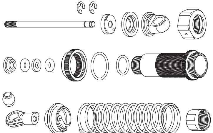
Rear Shock Absorber 2PCS
