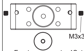
Front arm mount 1Set
