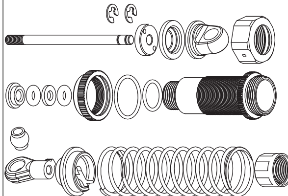
Rear Shock Absorber 2 Set
