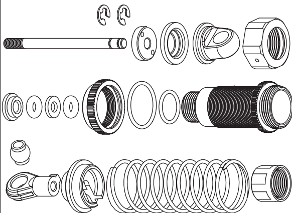
Front Shock Absorber 2 Set
