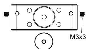
Front arm mount 1Set
